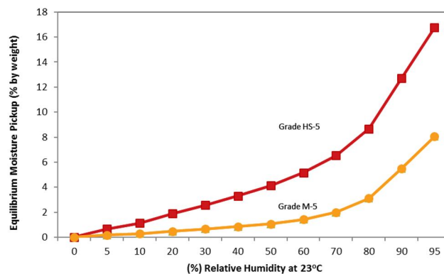
Moisture Adsorption by CAB-O-SIL® Hydrophilic Fumed Silica
